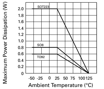
Power dissipation Derating
