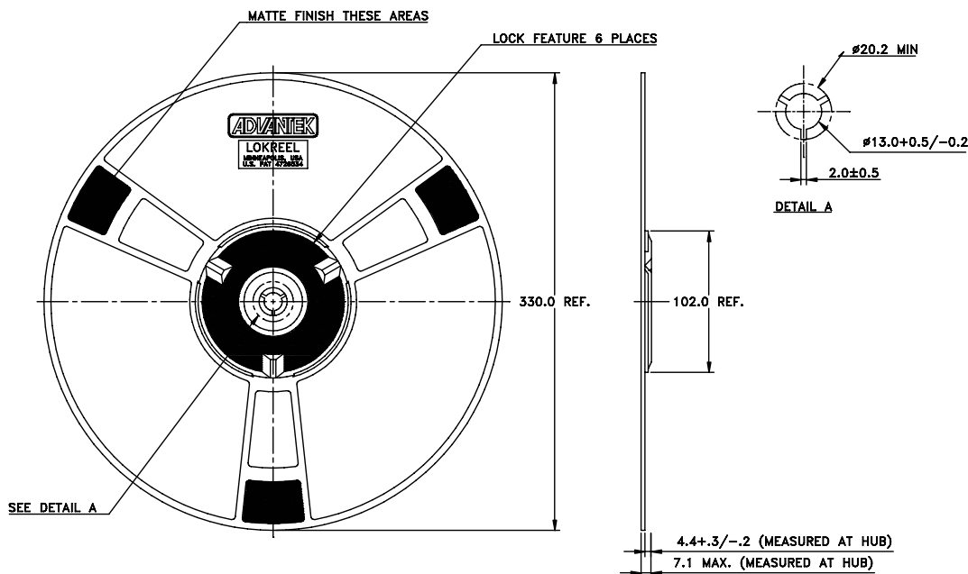
Figure 7: Carrier Tape
