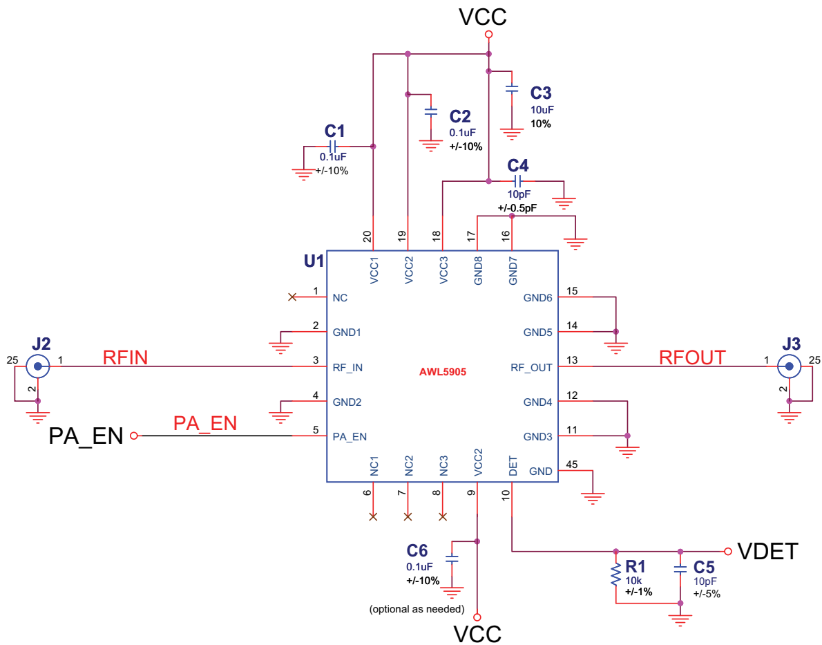
Figure 3: Application Circuit
