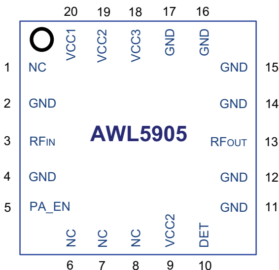
Figure 1: Pinout Diagram
