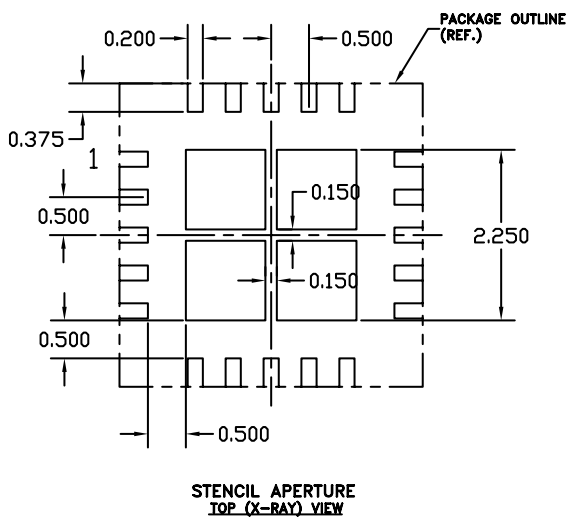
Figure 6: Recommended PCB Layout Information
