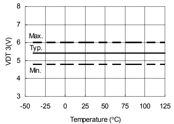
Figure 28. DT mode select Threshold (3) vs. Temperature
