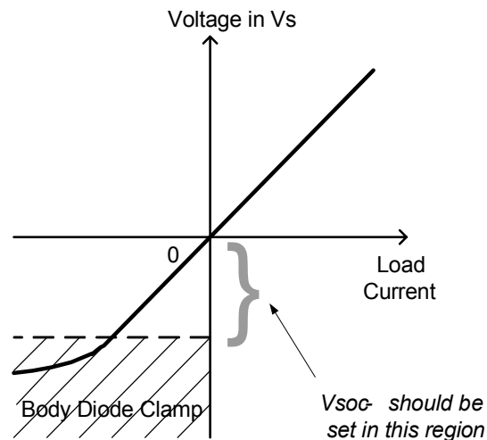
Figure 13. Body Diode in MOSFET Clamps vs Voltage
