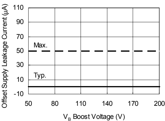
Figure 14B. Offset Supply Leakage Current vs. Supply Voltage
