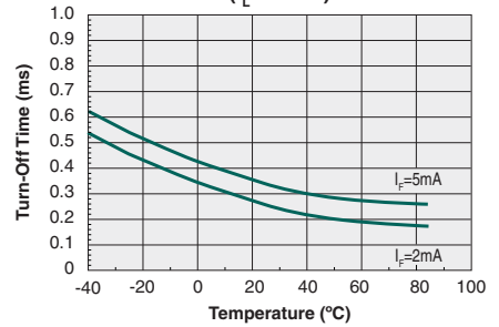
Typical Turn-Off Time vs. Temperature ( I_L=50mA )
