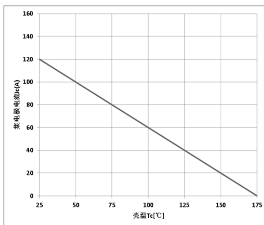
Figure 16. Collector Current-Tc Characteristics
