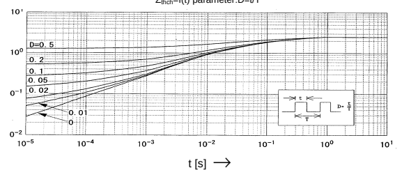
Transient Thermal impedance
