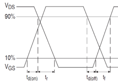
Fig 24b. Switching Time Waveforms
